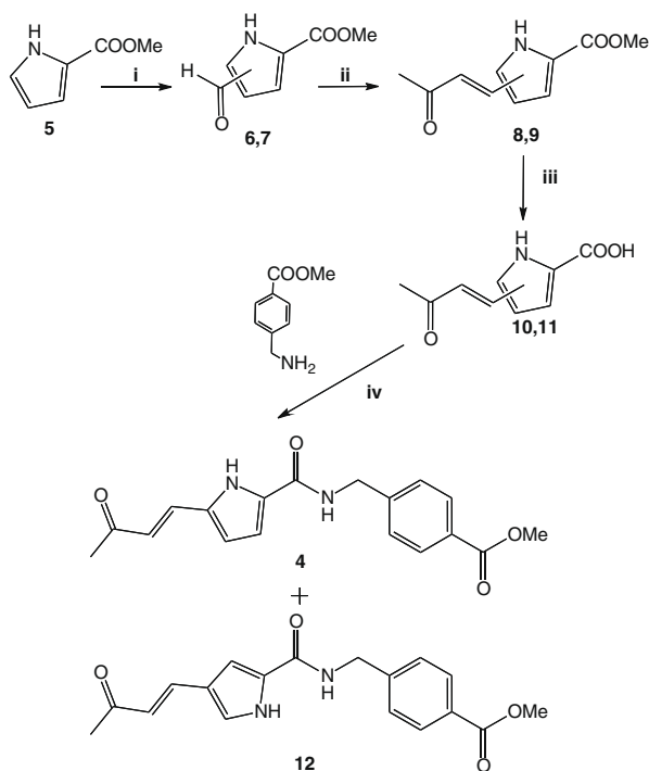
Scheme 1. Reagents and conditions: (i) DMF, POCl 3 reflux 15 m; (ii) acetone, pyrrolidine 30%, H 2 O; (iii) KOH, MeOH reflux 15 h; (iv) EDCl, DMAP, rt, on.
